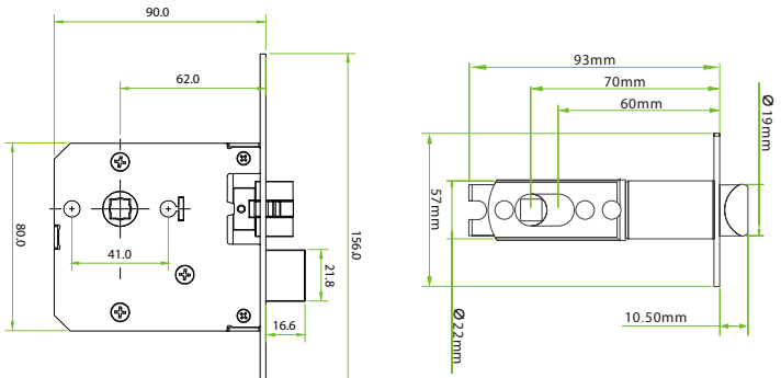
German Standard Mortise American Standard Mortise
